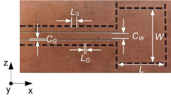
Figure 3.2-2: Fabricated SIW cavity resonator at 12 GHz.
