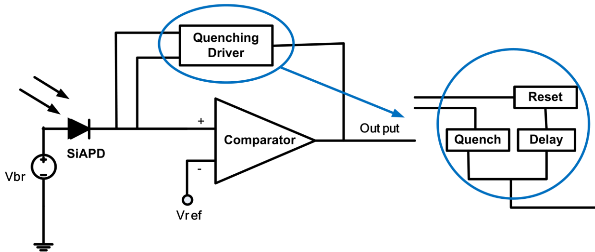
Figure 2.4: Active Quenching Circuit
