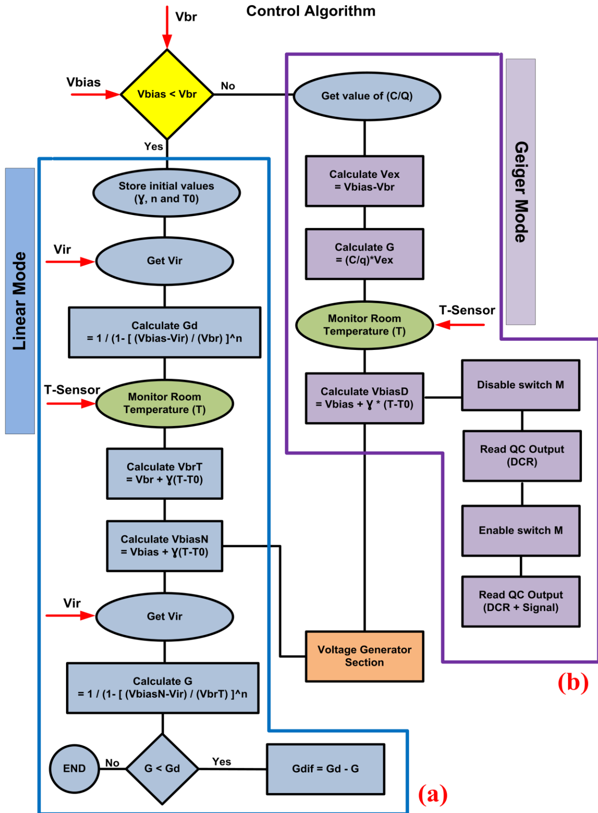
Figure 3.12: Control algorithm to compensate the thermal effect: (a) Linear-mode Algorithm, (b) Geiger-mode Algorithm
