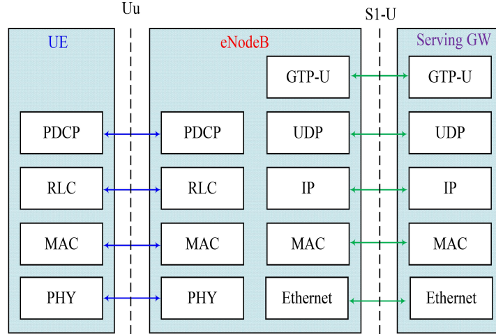
Figure 2.2 User Plane Protocols.
