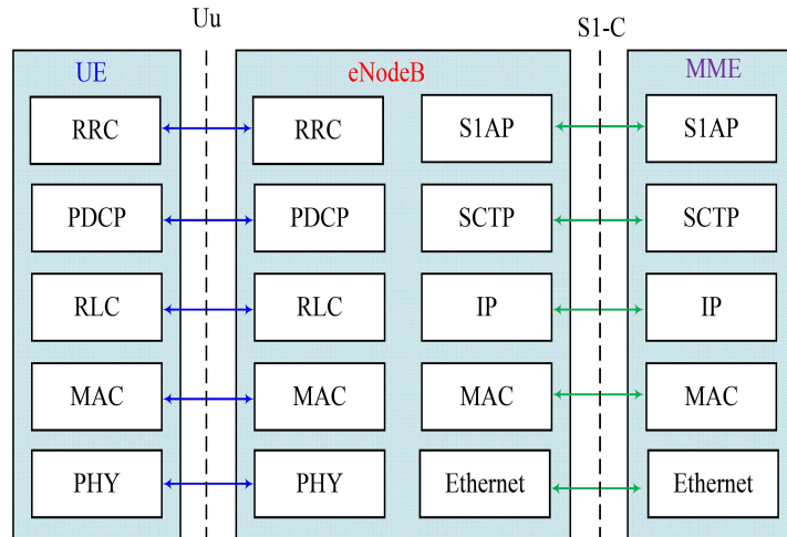
Figure 2.3 Control Plane Protocols.
