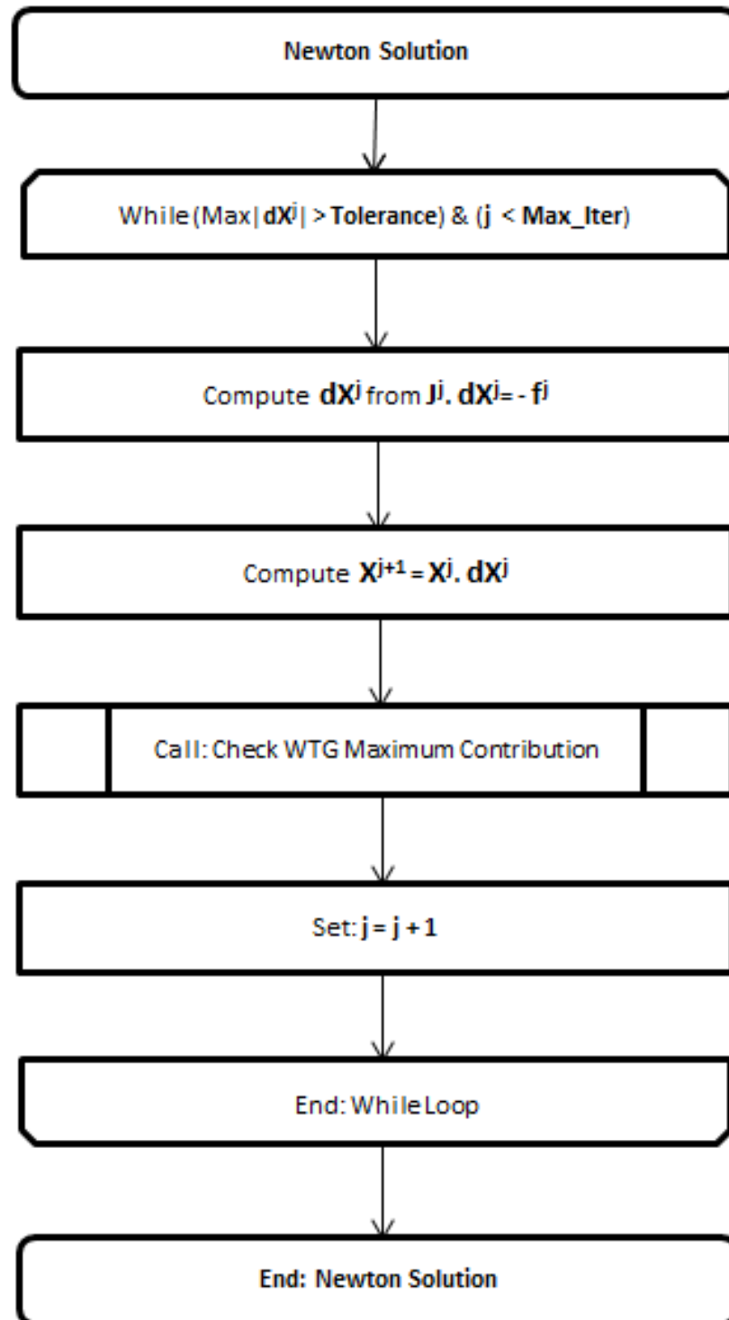
Figure 5-6 : Fault-flow algorithm
