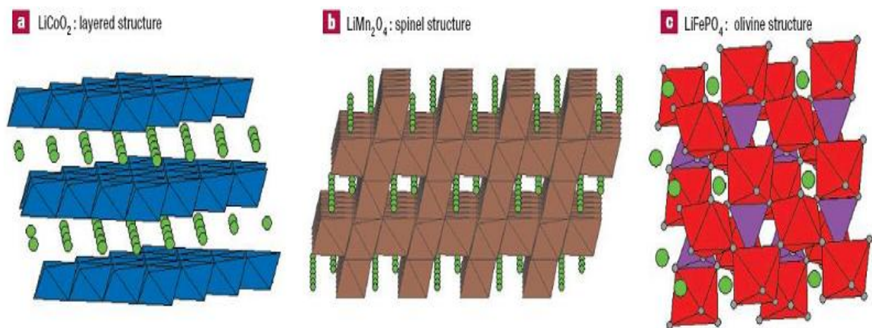
Figure 2-2: The crystal structure of (a) a layered type of \text{LiCoO}_2 , (b) a spinel type of \text{LiMn}_2\text{O}_4 , and (c) an olivine type of \text{LiFePO}_4 . Li: green, Co: blue, Mn: brown, Fe: red, and P: purple [36]
