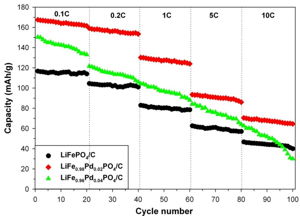
Figure 6-9: Cycling performance of \text{LiFePO}_4/\text{C} , \text{LiFe}_{0.98}\text{Pd}_{0.02}\text{PO}_4/\text{C} and \text{LiFe}_{0.96}\text{Pd}_{0.04}\text{PO}_4/\text{C} samples at various discharge rates
