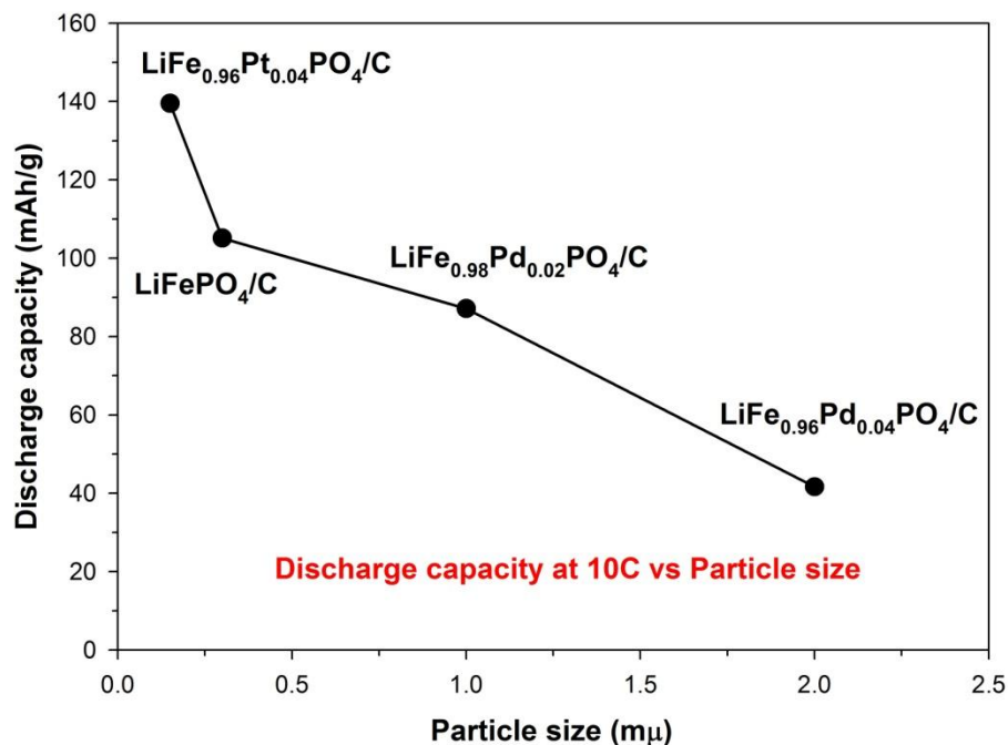
Figure 7-4: Specific discharge capacities at 10C rate of doped- \text{LiFePO}_4/\text{C} materials prepared by sol-gel vs their particle size
