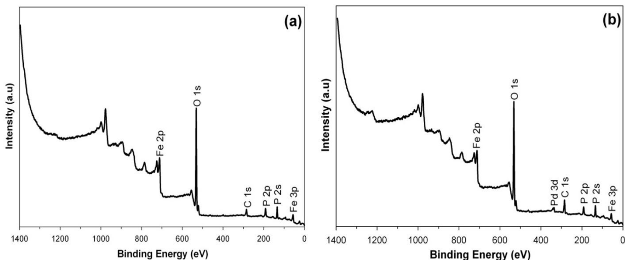
Figure 5-2: XPS spectra of the samples: (a) LiFePO 4 ; and (b) LiFe 0.96 Pd 0.04 PO 4
