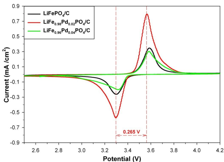
Figure 6-7: CV curves of \text{LiFePO}_4/\text{C} , \text{LiFe}_{0.98}\text{Pd}_{0.02}\text{PO}_4/\text{C} and \text{LiFe}_{0.96}\text{Pd}_{0.04}\text{PO}_4/\text{C} samples at scanning rate of 0.1 mV/s
