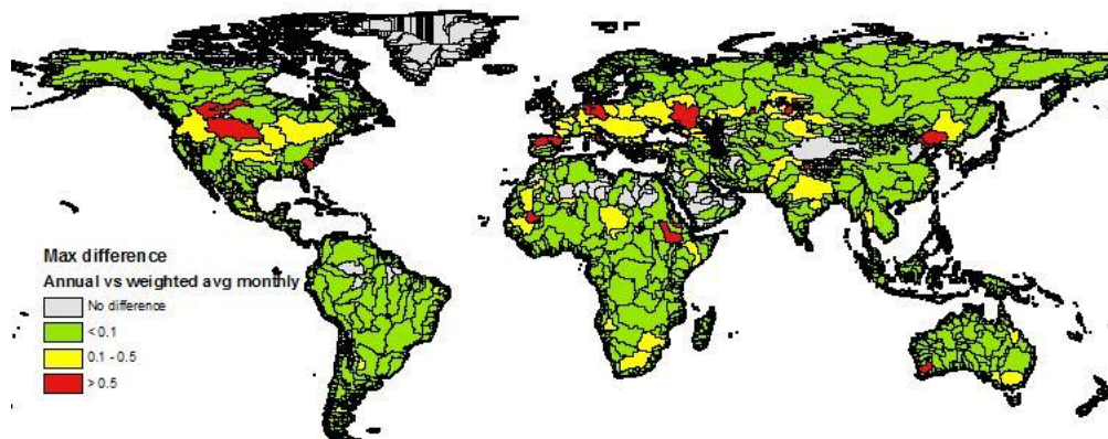
Fig.S5: Difference between annual scarcity indicators calculated from annual data vs. from a withdrawal-based weighted average of monthly data. Results are obtained with M-PfisterSc which scarcity indexes range from 0.01 to .1
