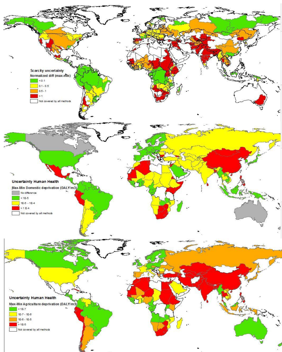
Figure 5-11 Uncertainty associated with the choice of model for a) scarcity, b) domestic water deprivation and c) agricultural water deprivation.
