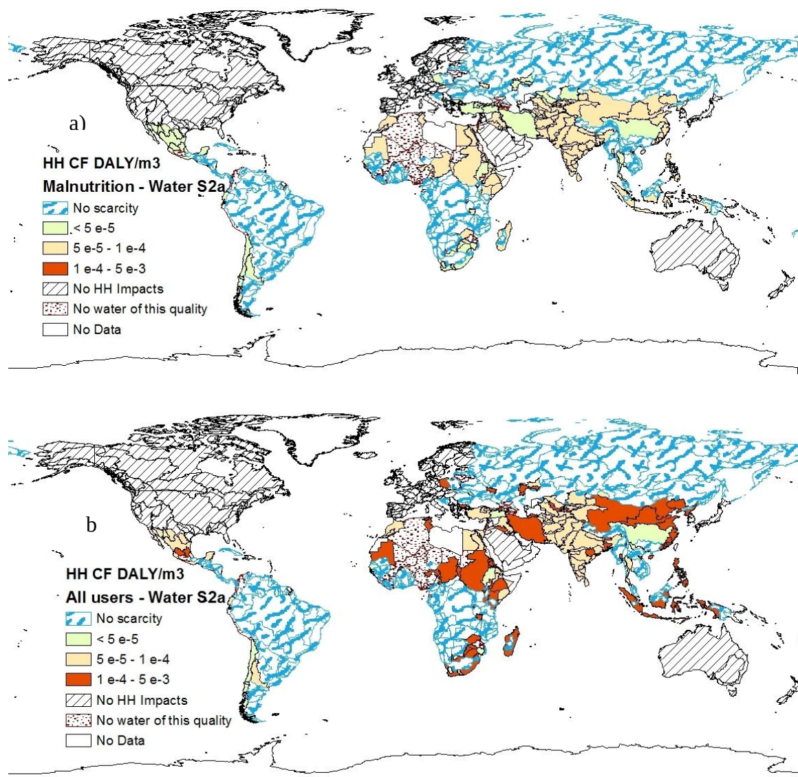
Figure 4-4 Human health characterization factors for good quality surface water (category S2a) in DALY/m³ a) considering that agriculture is the only marginal user affected (along with fisheries), leading therefore to malnutrition and b) considering all users are affected proportionally to their use (i.e. also including domestic users and therefore considering health burdens due to lack of hygiene and sanitation in addition to malnutrition).
