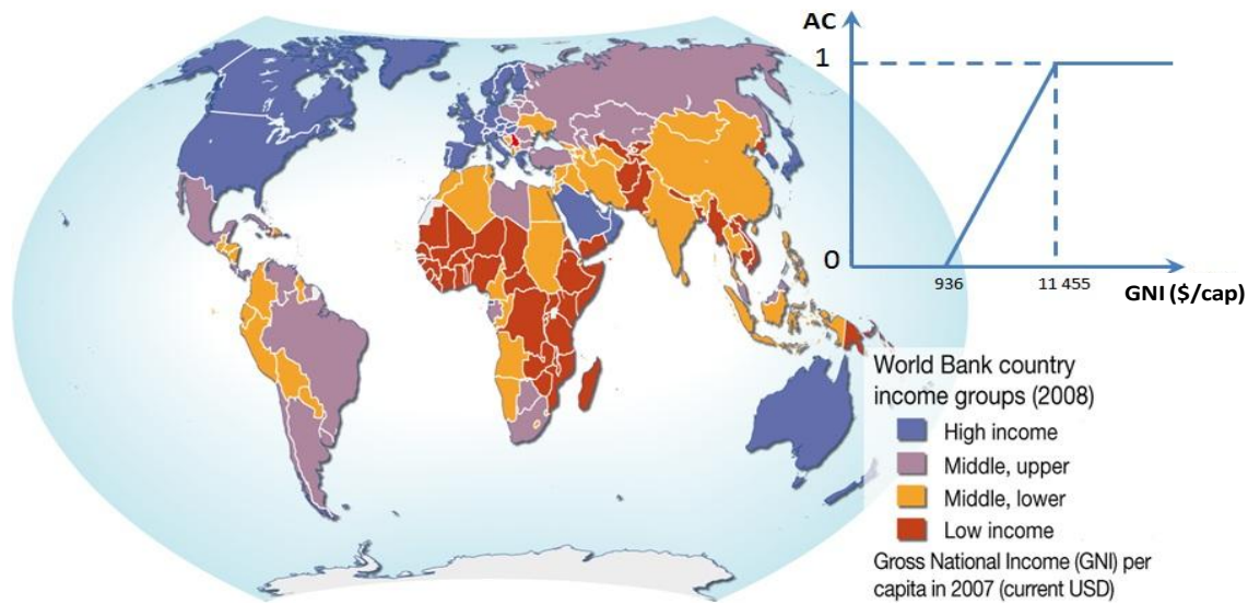
Figure 4-2 Adaptation capacity based on World Bank country classification: No adaptation for low-income countries, complete (100%) adaptation for high-income countries and partial adaptation for middle-income countries
