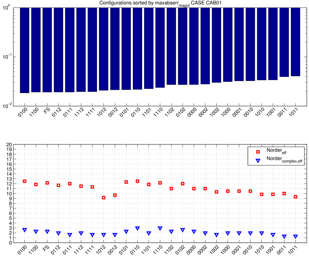
Figure 5.8: W/magVF MAE_2 results in the phase domain, all configurations, CAB01
