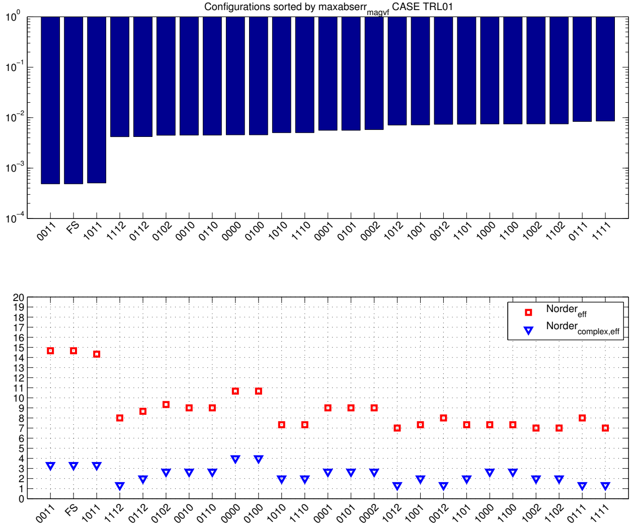
Figure 5.12: W/magVF maxabserr results in the phase domain, all configurations, TRL01
