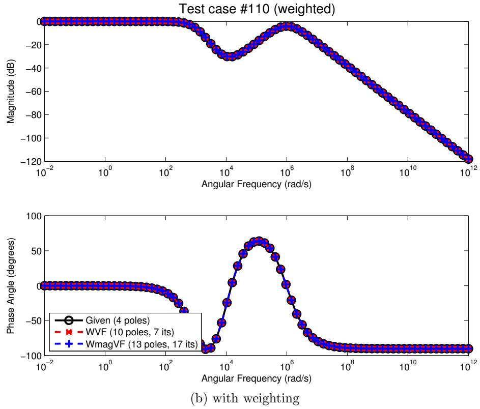
Figure 4.8: Repeated poles, with increased order. Actual order is 4 (2 repeated real poles and one pair of complex conjugate poles)
