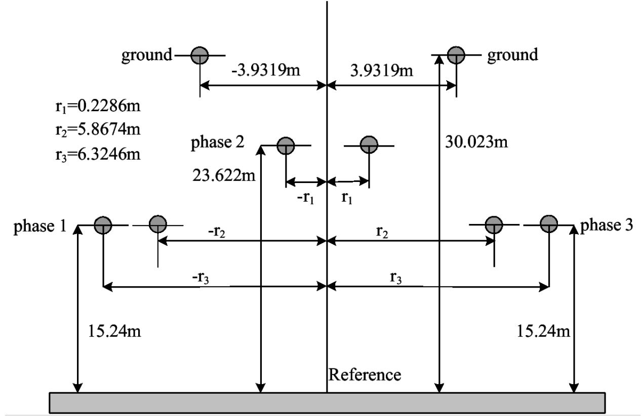
Figure 5.3: Configuration of overhead transmission lines studied, TRL01 case
