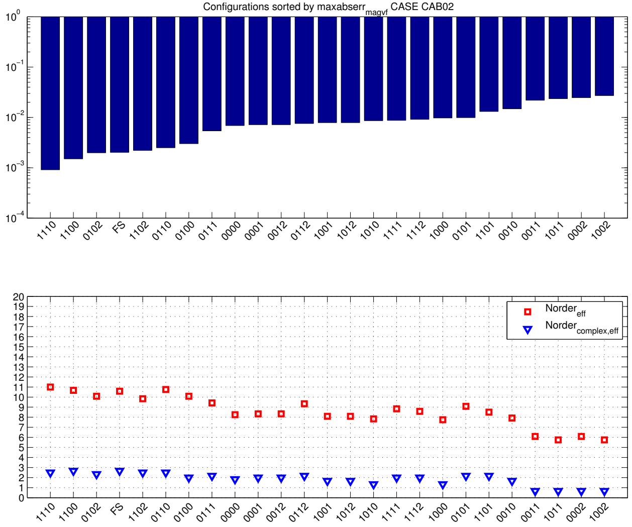
Figure 5.10: W/magVF maxabserr results in the phase domain, all configurations, CAB02
