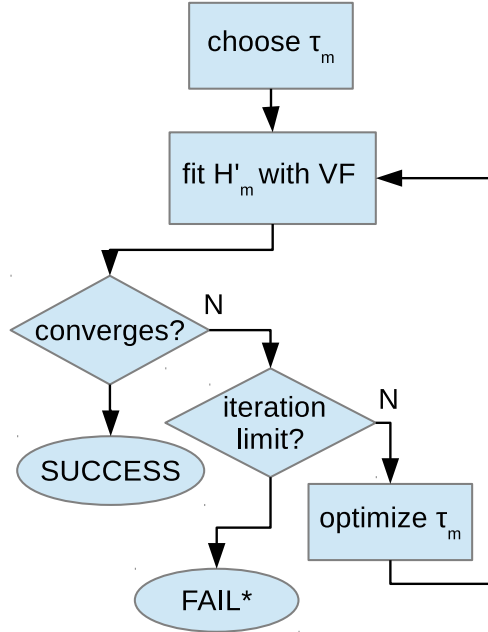
Algorithm 5.1 Algorithm for fitting H'_m using VF or WVF
