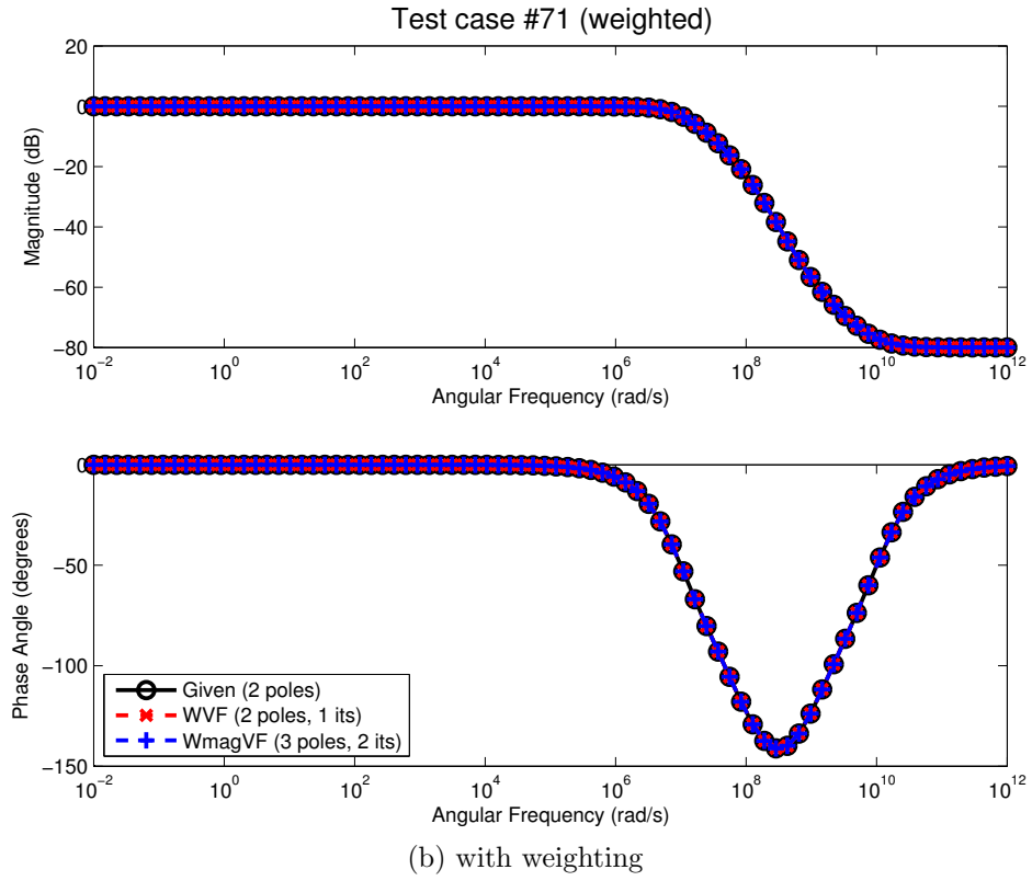
Figure 4.4: Biproper transfer function test case (Case #71), using biproper settings in the fitters, asymflag = 2
