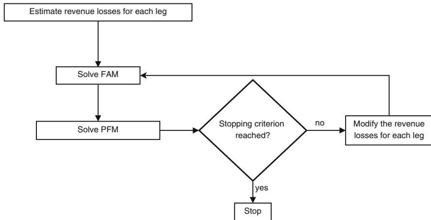
Fig. 2 The method of Dumas et al. (2009): fleet assignment with external PFM reevaluation
