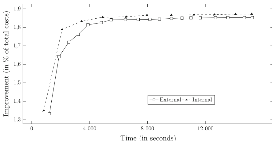
Fig. 4 Average results of the internal and external methods (5,180-leg network)
