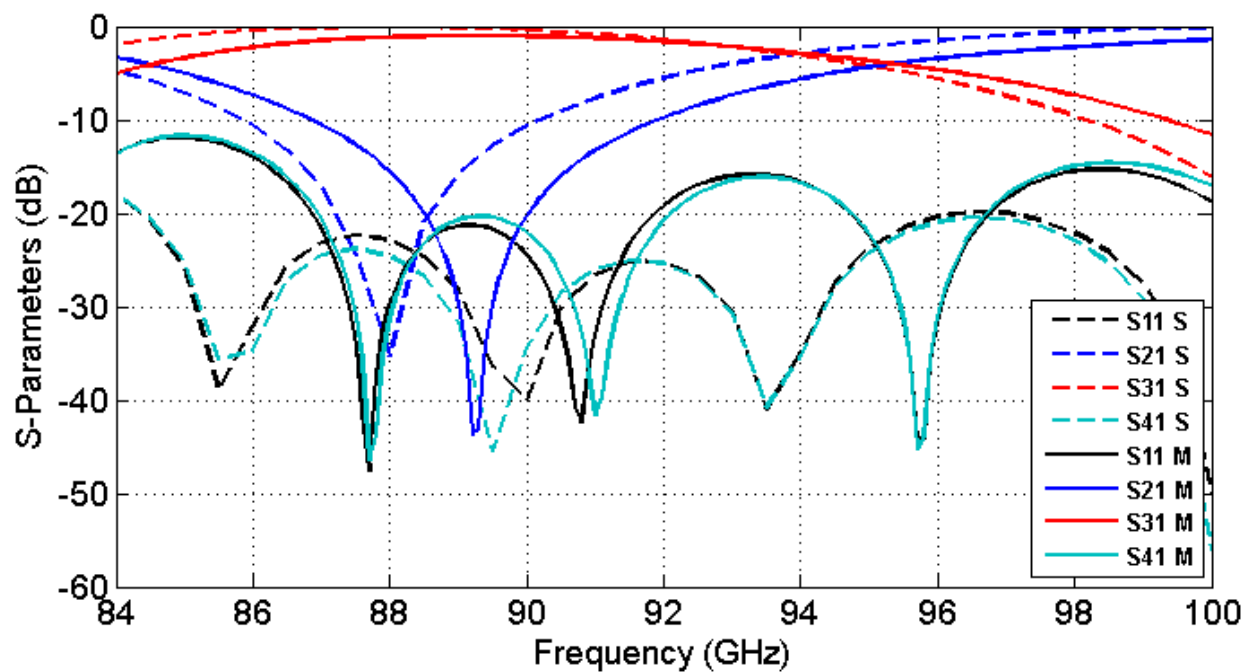
Figure 3-33: Simulated (S) and measured (M) S-parameters of the TE_{20} mode Type B iSINRD coupler, including the 88 GHz cross-over coupling.
