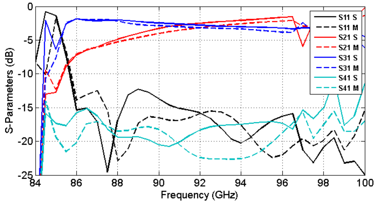
Figure 3-34: Simulated (S) and measured (M) S-parameters of the asymmetric iSINRD-iSIW coupler, including the cross-over coupler ( TE_{20} operation).
