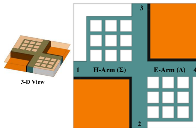
Figure 4-12: A 3-D view (left) and a top view of the asymmetric iSINRD cruciform magic-T.
