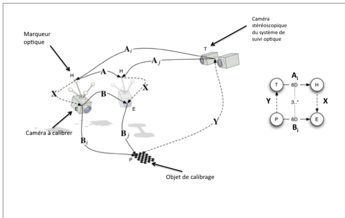
Figure 1.25 Le calibrage bras-œil
