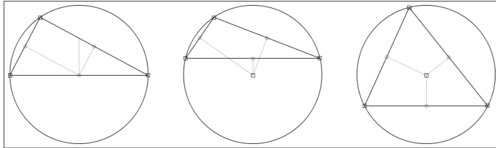
Figure 2.5 Cercle circonscrit
