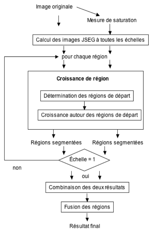
Figure A.9 Algorithme de segmentation
