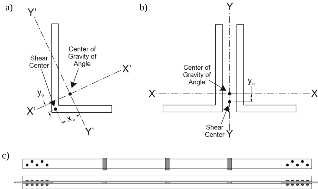
Figure 1.4: Properties of angle cross-sections and built-up brace: a) single angle; b) double angle; c) double angle brace
