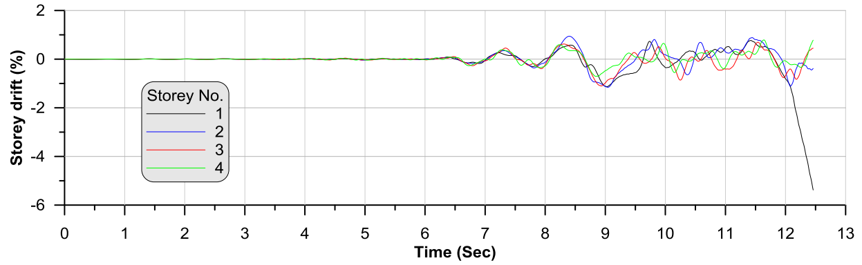
Figure I. 24: Inter-storey drift for CBF retrofit+exp. model under earthquake NGA-787 with F_{sm} 1.1
