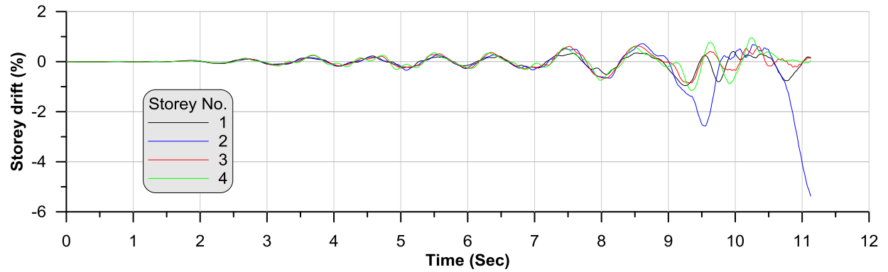
Figure I. 22: Inter-storey drift for CBF retrofit+exp. model under earthquake NGA-762 with F_{sm} 1.2
