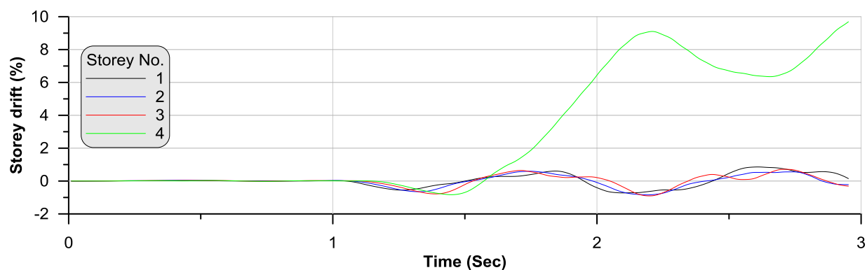
Figure I. 2: Inter-storey drift for CBF_{\text{design+exp.}} model under earthquake NGA-57 with F_{sm} 1.2
