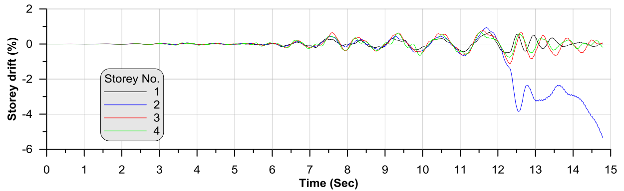
Figure I. 23: Inter-storey drift for CBF retrofit+exp. model under earthquake NGA-776 with F_{sm} 0.8
