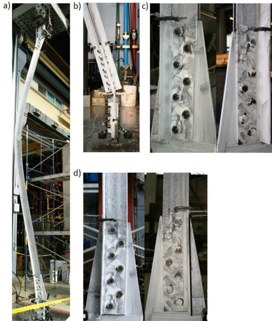
Figure 3.23: Specimen No. 2 - Observed behaviour during the test: a) Buckling of the brace; b) out-of-plane bending about gusset plate hinge; c) yielding on net section; d) in-plane bending of the brace in the connection region
