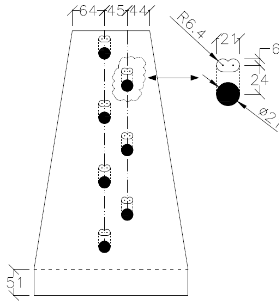
Figure 2.13: Increasing ductility and controlling force by reducing area in shear
