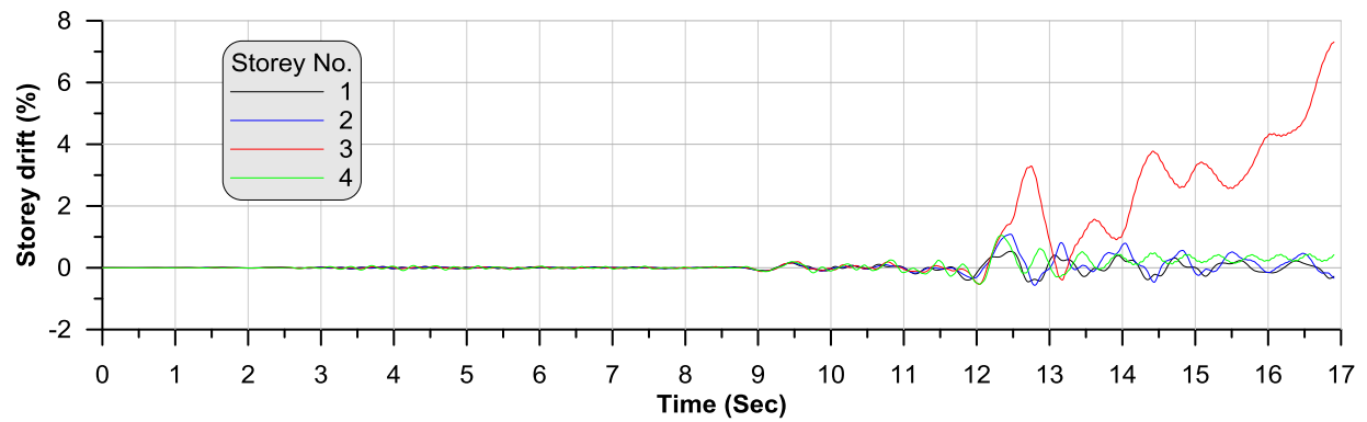
Figure I. 25: Inter-storey drift for CBF retrofit+exp. model under earthquake NGA-796 with F_{sm} 0.9
