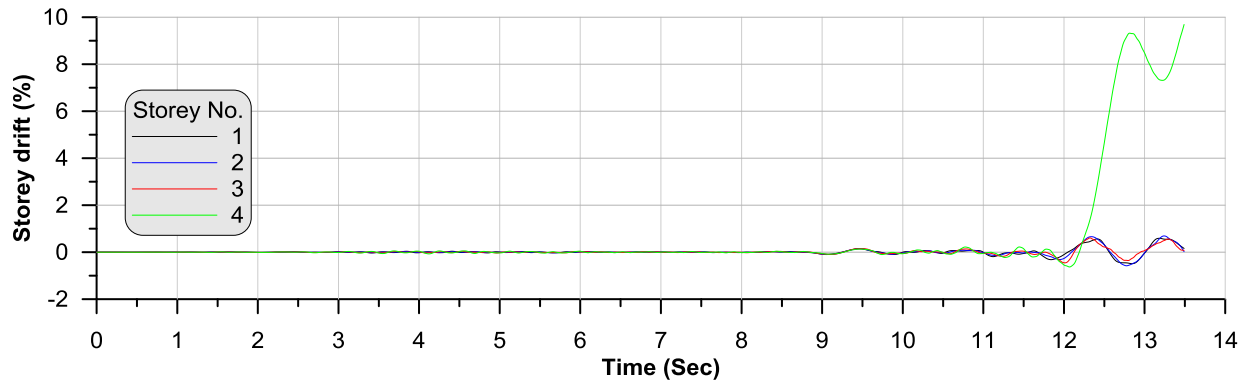
Figure I. 16: Inter-storey drift for CBF design model under earthquake NGA-796 with F_{sm} 0.8
