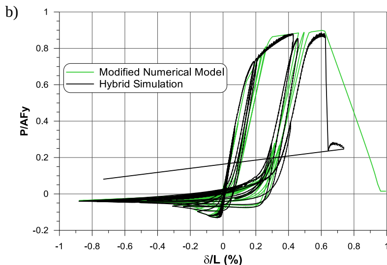
Figure 5.16: Comparison between modified numerical model analysis and hybrid simulation: a) Lateral displacement time history at the first-storey; b) Brace hysteretic response (continued)
