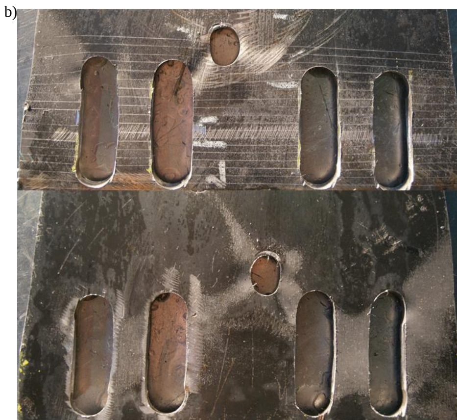
Figure 3.30: Specimen No. 3 - Observed behaviour of gusset plate in the region with slotted holes after test: a) gusset plate at bottom; b) gusset plate at top (continued)
