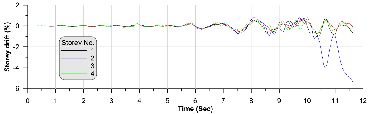
Figure I. 26: Inter-storey drift for CBF retrofit+exp. model under earthquake NGA-807 with F_{sm} 1.2
