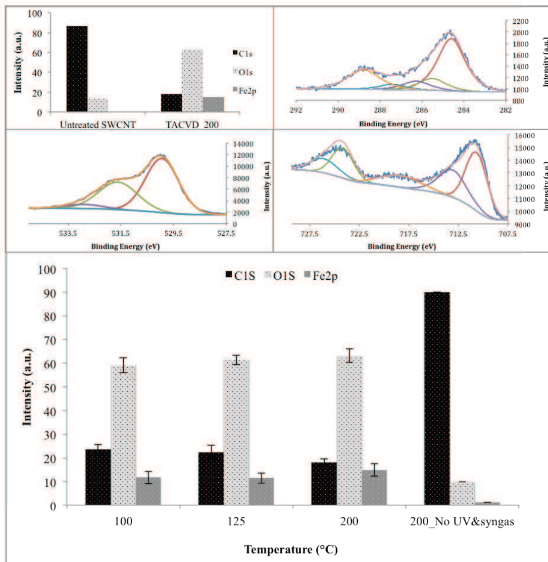
Fig. S3. A) Survey XPS spectra of treated SWCNT by syngas/TACVD_200 C, B) C1s HR-XPS of SWCNT treated by syngas/TACVD_200 C, C) O1s HR-XPS of SWCNT treated by syngas/TACVD_200 C, D) Fe2p HR-XPS of SWCNT treated by syngas/TACVD_200 C, E) Over plot of survey XPS spectra treated SWCNTs by syngas over heating (the inset table is presenting the related numbers).
