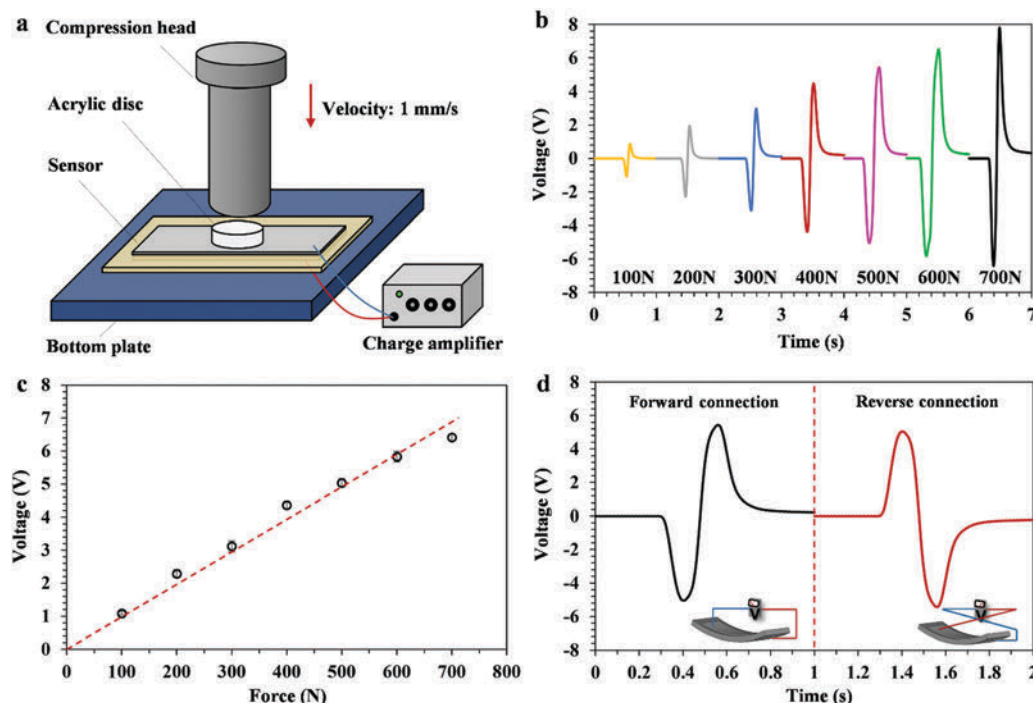
Fig. 4 Compression test. (a) Schematic of the compression test setup. (b) Voltage curves during a 1 s period. (c) Maximum voltage generated by a 40 × 20 mm printed piezoelectric PVDF sensor ( R = 4 ) under the maximum compressive forces of 100, 200, 300, 400, 500, 600 and 700 N. Error bars indicate the standard deviations obtained from three measurements. (d) Switching-polarity test: voltage generated during a 1 s period under the compression of 500 N using forward and reverse connections.
