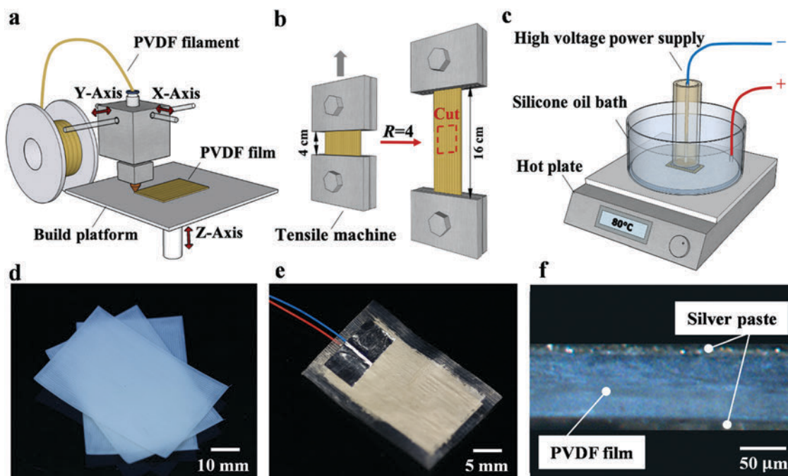
Fig. 1 Fabrication of the piezoelectric PVDF films. Schematic of the (a) FFF printing process of the PVDF films (60 × 40 × 0.15 mm). (b) Stretching process of the printed PVDF films ( R = 4 ). (c) Contact poling process of the stretched PVDF films (40 × 20 × 0.06 mm). Photos of (d) FFF printed PVDF films. (e) A piezoelectric PVDF film with electrical connections. (f) Optical image of the cross-section of the piezoelectric PVDF film.
