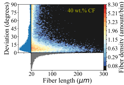
Figure 12: 2D histogram representation of the correlated lengths and angle of deviation from tracking direction (z) for fibers present in a PEEK specimen with 40 wt.% CF filling ratio. Single-variable histograms are juxtaposed on the left-hand and lower side, to highlight the relationship between the counts for each variable and the correlated density values.
