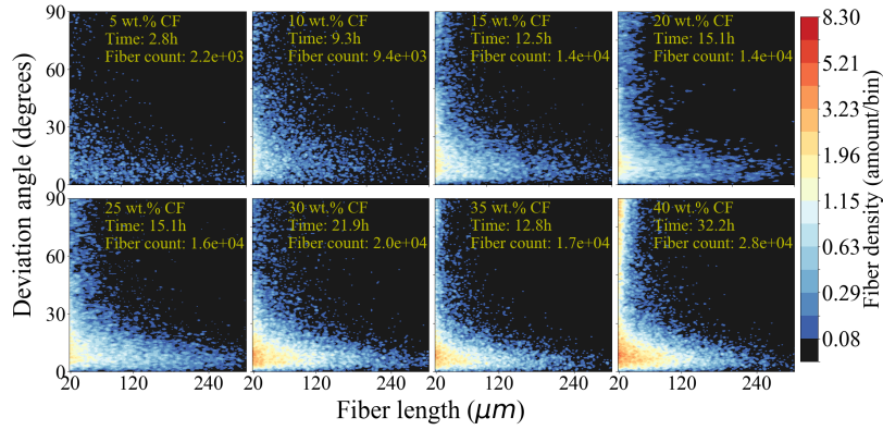
Figure 13: Correlated lengths and deviation histograms for PEEK SFRP with filling ratios of 5-40 wt.% CF. For all levels of filling, there exists an inverse correlation between fiber length and deviation: longer fibers will be more aligned with the extrusion direction. Processing time is given, along with fiber count for each scan.
