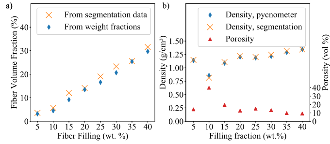
Figure 10: Experimental validation: a) Comparison of fiber volume fraction obtained directly from the segmentation output, vs. calculated from the known densities of matrix and reinforcement materials, as a function of fiber filling fraction. The difference between the two is at most 4% (meaning if one method gives 10%, the other can give at most 14%). b) Comparison of specimen density, as calculated from the segmentation output and the density measured directly with the help of a gas pycnometer. Very high agreement (mean error <2\% ) between the two indicates the proportions of matrix, fiber and porosity as predicted by the segmentation are a reliable indicator of the proportions in the real material. The porosity measurement (obtained from segmentation) is presented, to highlight the success of OpenFiberSeg even with vastly dissimilar morphologies (porosity ranging from 10 to 40 vol%).
