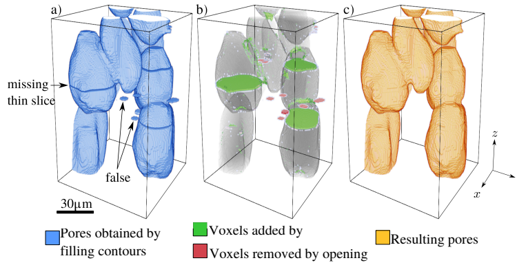
Figure 3: Porosity labelling, typical region of data (2D slicing in x-y planes): a) as obtained by filling the closed contours of the Canny algorithm. b) Morphological closing fills in missing thin slices inside well-defined pores, opening removes false detections. c) Resulting pores.
