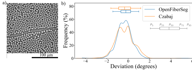
Figure 8: Extraction performed on original micro-CT scan of unidirectional graphite/epoxy composite. a) Sample data slice, reproduced with authorization [35]. b) Probability density function of fiber deviation from main direction, as reported by original authors, and as measured with OpenFiberSeg. The box and whisker plots for each peak represent the 5 th , 25 th , 50 th , 75 th and 95 th percentiles for both segmentation methods, which are all within 0.5°, indicating good agreement between the methods.
