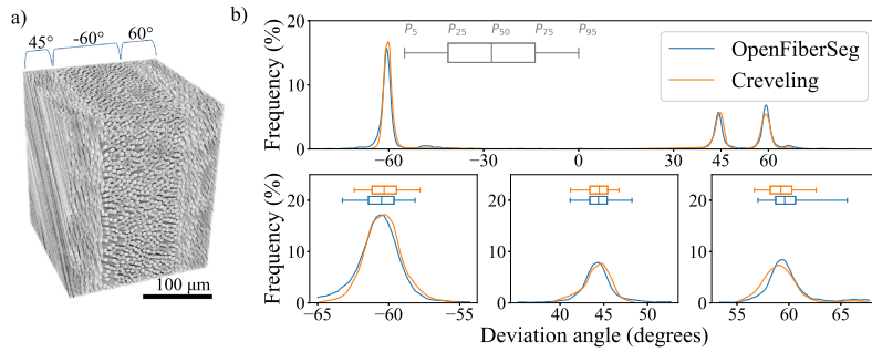
Figure 9: Extraction performed on micro-CT scan of carbon/epoxy laminate. a) rendering of original data, showing the main angles of the three layers, relative to the vertical direction [36]. Reproduced with authorization. b) Probability density function of fiber deviation from main direction, as reported in [36], and as measured with OpenFiberSeg. The bottom portion shows zoom around the three main peaks, with generally good agreement between the output of the two methods. The box and whisker plots for each peak represent the 5 th , 25 th , 50 th , 75 th and 95 th percentiles for both segmentation methods, when grouping the data around the three main peaks.
