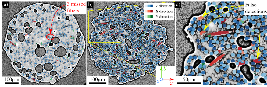
Figure 11: Output of segmentation for 2 material compositions: a) PEEK with 15 wt.% CF and in b) with 40 wt.% CF. Different colormaps are used to represent in which reference direction the fiber was detected. The majority are detected in the out-of-plane (z direction), and some in the in-plane directions x and y. In c), a closer look shows that more false detections are present in the x direction, but the strongly inclined fibers are also successfully captured.
