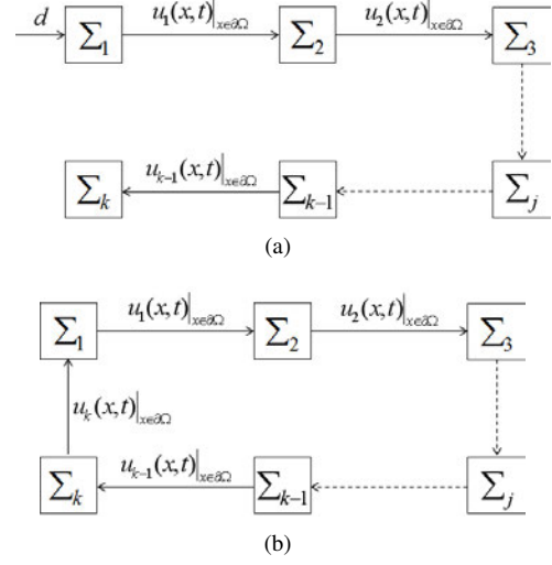
Fig. 1. Systems coupled on the boundary: (a) Systems coupled via (18); (b) Systems coupled via (19).
