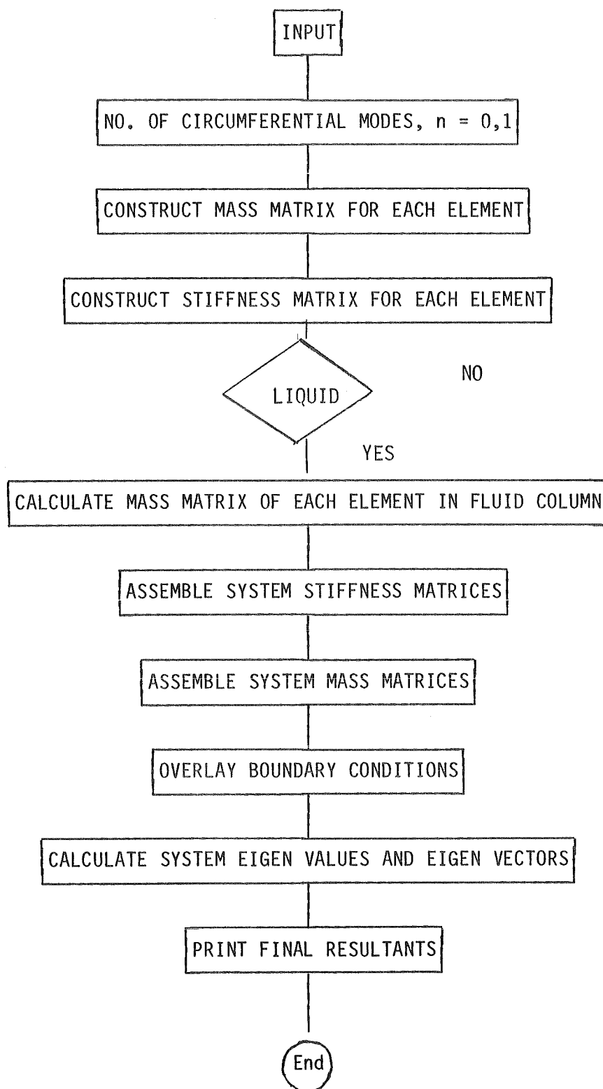
FIGURE 6 - Slow chart of the principle program
