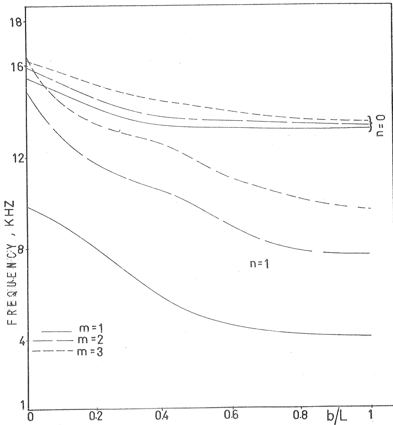
FIGURE 15 - VARIATION IN FREE VIBRATION OF A CYLINDRICAL SHELL PARTIALLY FILLED WITH LIQUID AND SIMPLY SUPPORTED AT BOTH ENDS ( \rho_l = 0.935 \times 10^{-4} \text{ lb} - \text{sec}^2 / \text{in}^4 )
