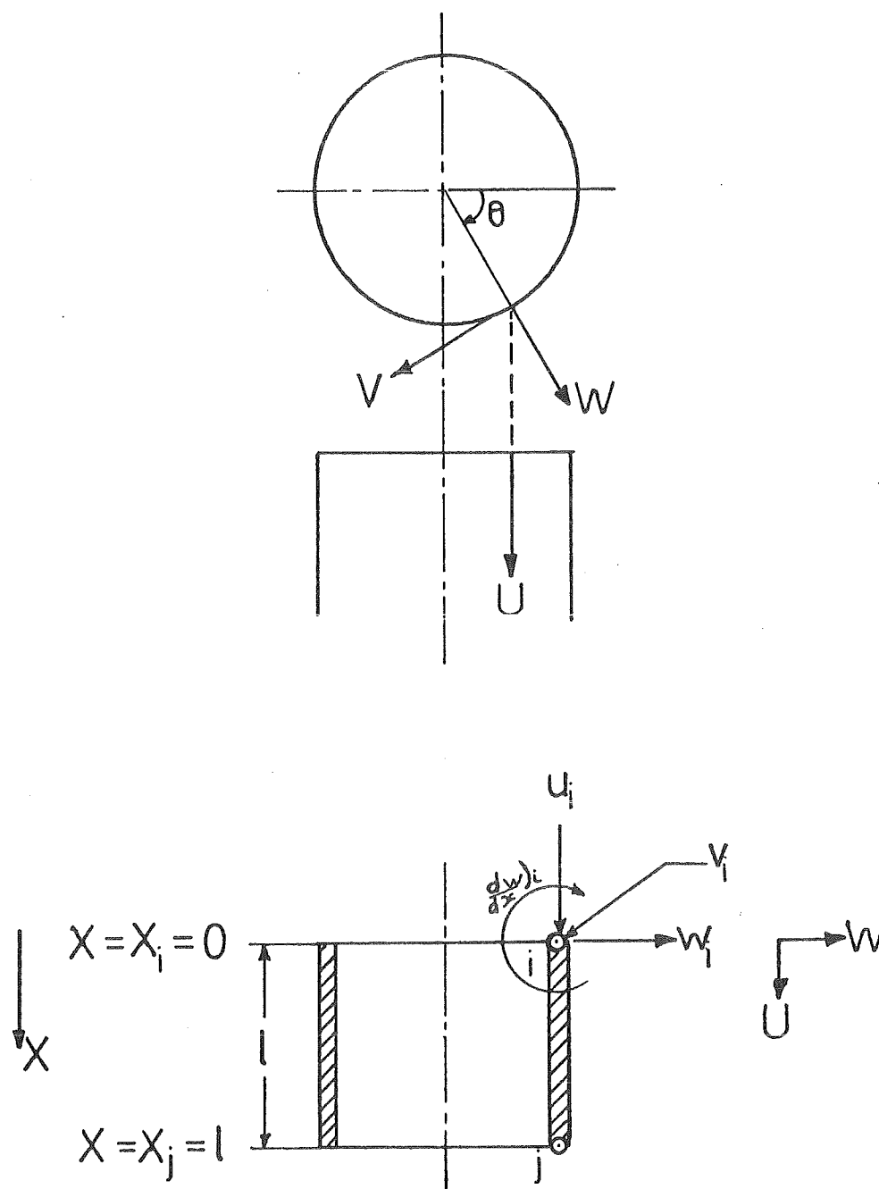
FIGURE 3 - NODAL DISPLACEMENTS AT JOINTS i AND j
