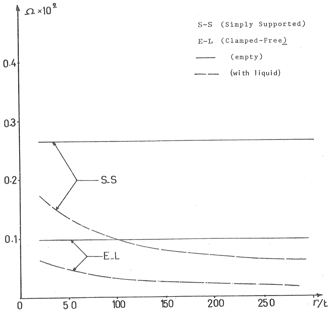
FIGURE 13 - EFFECT OF THE LIQUID ON VIBRATION PARAMETER ( \Omega )
