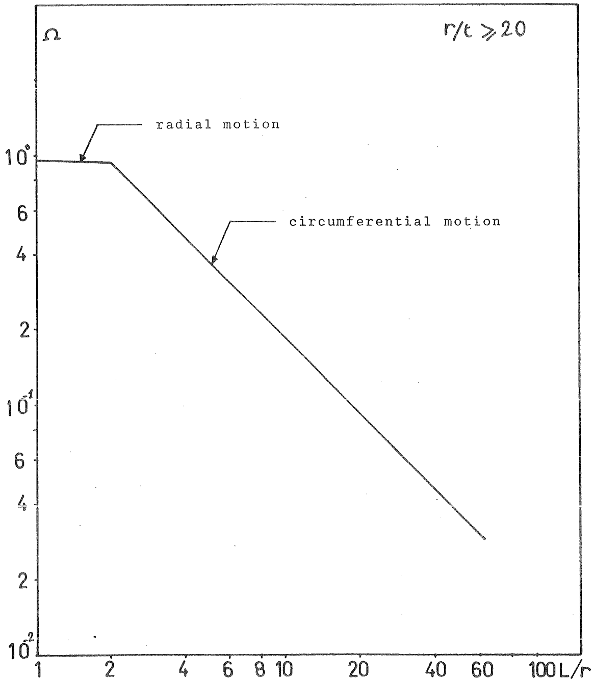
FIGURE 12 - VARIATION OF VIBRATION PARAMETER ( \Omega ) IN CONJUNCTION WITH L/r OF A CYLINDRICAL SHELL SIMPLY SUPPORTED AT BOTH ENDS
