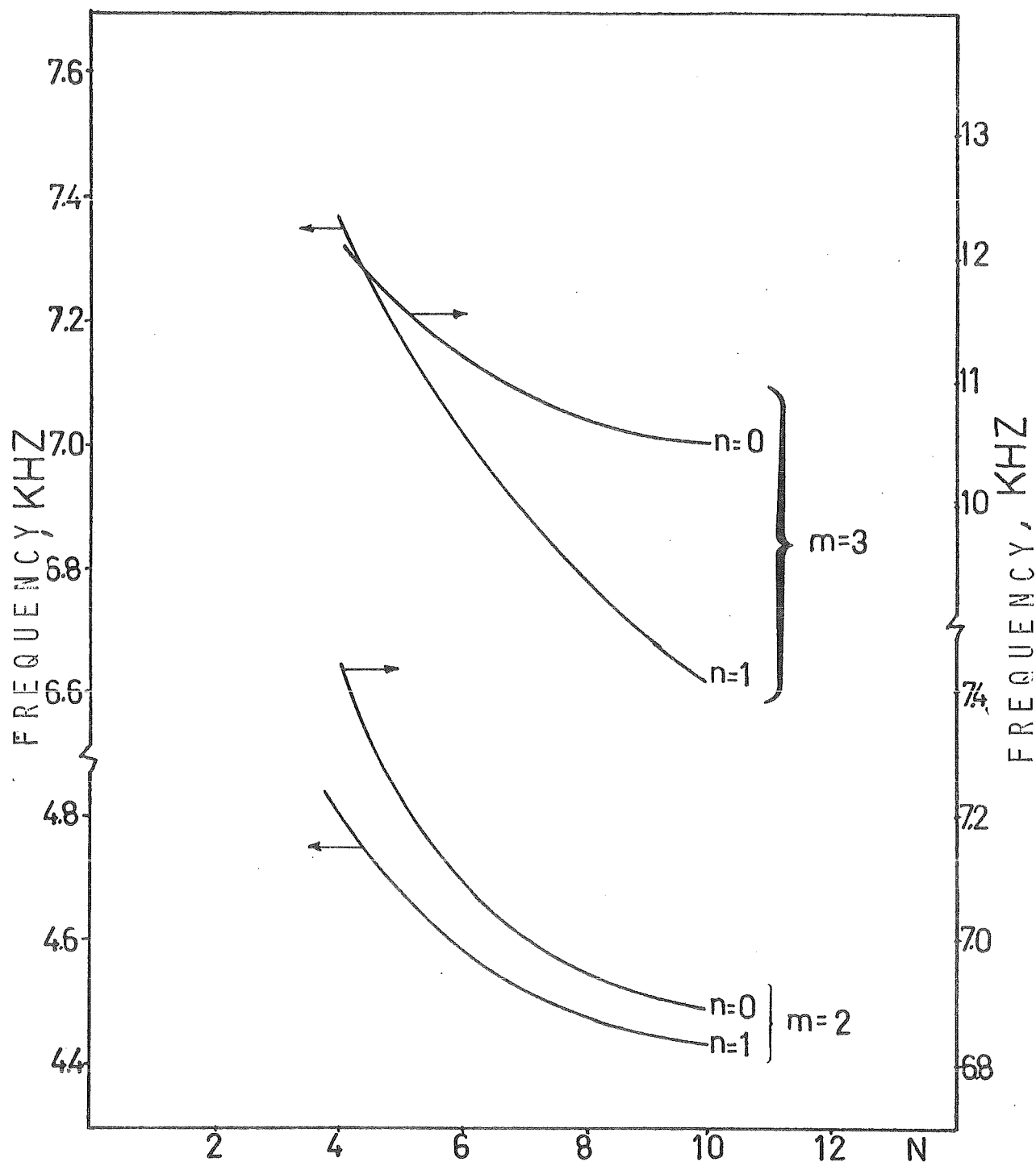
FIGURE 8b - CONVERGENCE TEST OF A CYLINDRICAL SHELL SIMPLY SUPPORTED AT BOTH ENDS FOR n = 0 and n = 1 ( N = number of finite elements)
