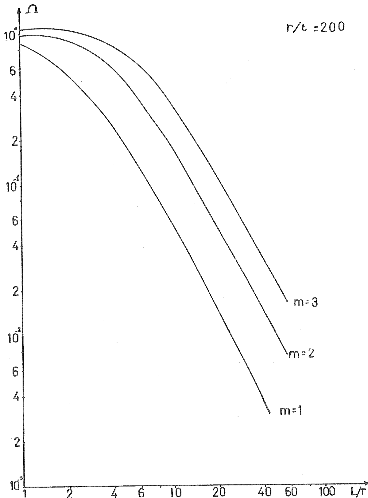
FIGURE 9 - VARIATION OF VIBRATION PARAMETER ( \Omega ) IN CONJECTION WITH L/r OF A CYLINDRICAL SHELL SIMPLY SUPPORTED
