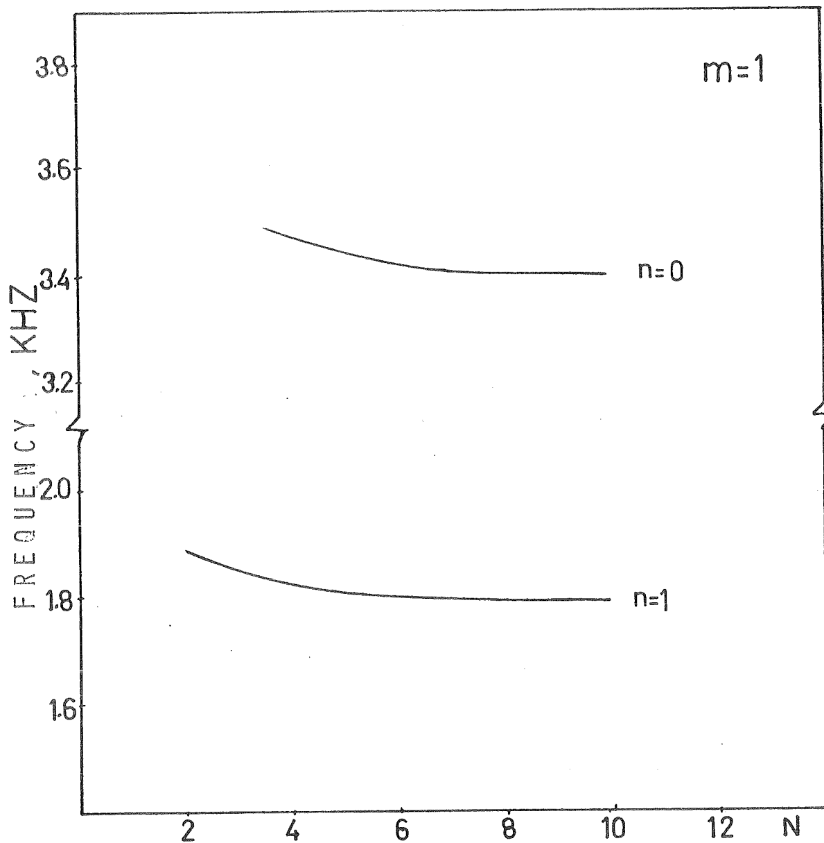
FIGURE 8a - CONVERGENCE TEST OF A CYLINDRICAL SHELL SIMPLY SUPPORTED AT BOTH ENDS FOR n = 0 and n = 1 ( N = number of finite elements)
