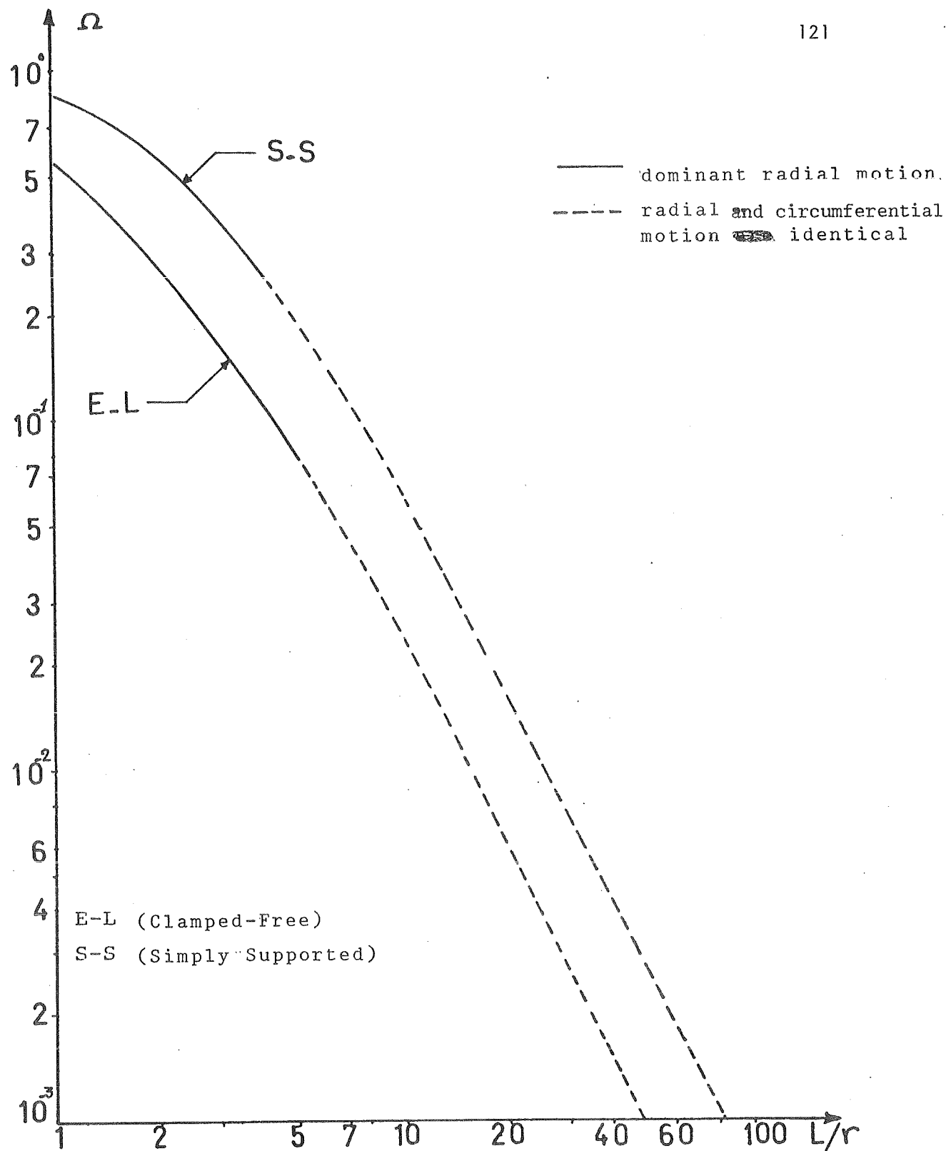
FIGURE 11 - EFFECT OF L/r ON EIGEN VALUES AND EIGEN VECTORS FOR DIFFERENT BOUNDARY CONDITION ( n = 1, m = 1, r/t = 100 and \Omega = \omega r \sqrt{\rho(1 - \nu^2)/E} )
