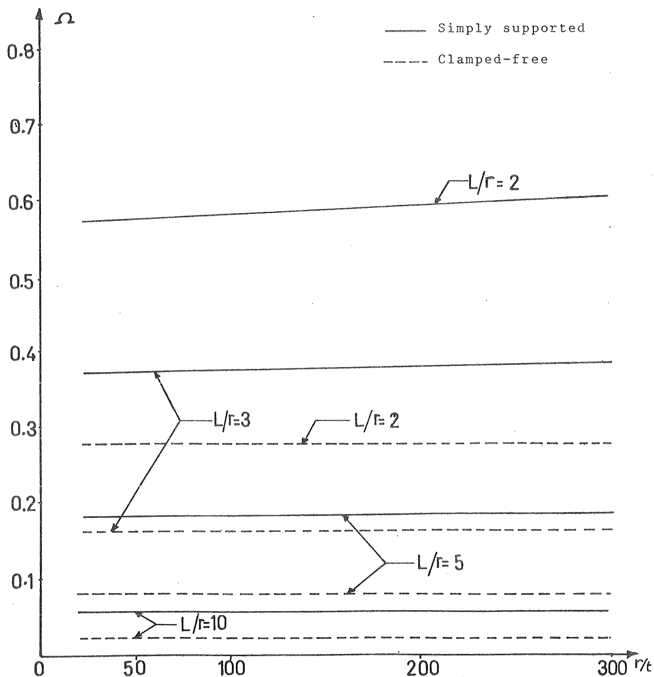
FIGURE 10 - VARIATION OF VIBRATION PARAMETER ( \Omega ) IN CONJUNCTION WITH r/t OF A CYLINDRICAL SHELL ( n = 1 , m = 1 , \nu = 0.3 and \Omega = \omega r \sqrt{\rho(1 - \nu^2)/E} )
