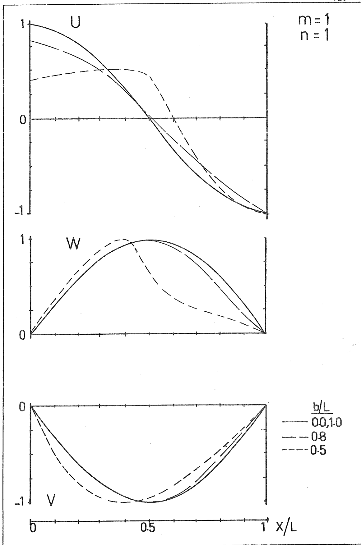
FIGURE 16 - NORMALIZED EIGEN VECTORS OF A SHELL SIMPLY SUPPORTED AT BOTH ENDS AND PARTIALLY FILLED WITH LIQUID
