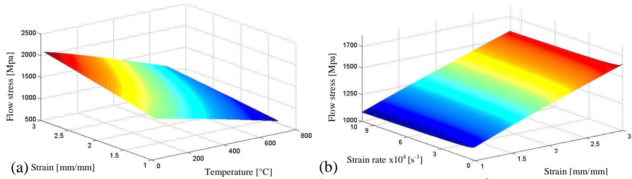
Figure 2.29- 3D representations of flow stress, a) At the strain rate of 10^4/s , b) At 400^\circ C
