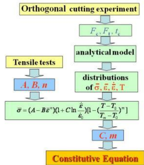
Figure 2.28- Development of the constitutive equation [40]
