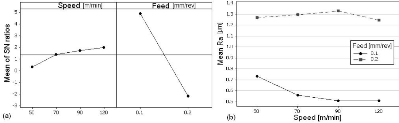
Figure 3: Surface roughness for carbide tool, (a) Sensitivity of speed on S/N ratio of Ra, (b) Ra measurements for different cutting conditions
