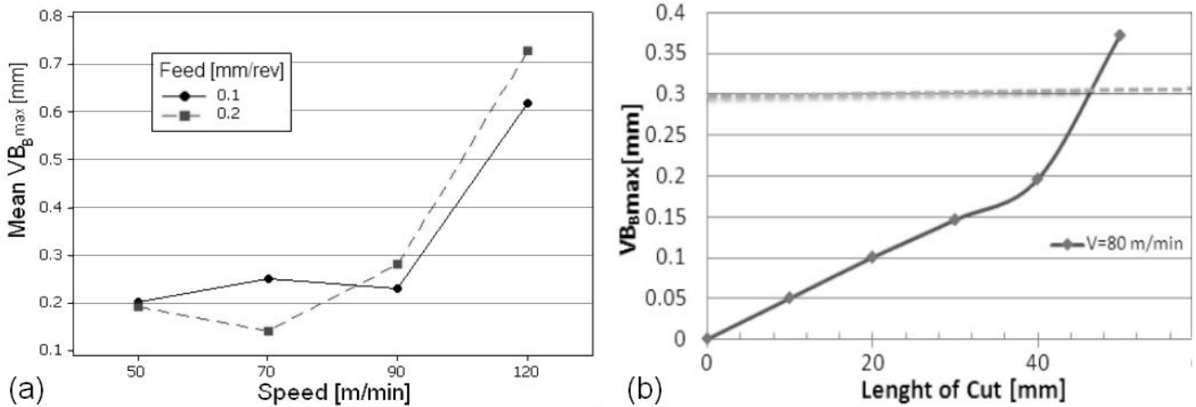
Figure 7: (a) Effect of cutting parameters on Carbide tool flank wear after L_c=40 mm, (b) tool wear progression at cutting speed=80 m/min and feed=0.1 mm/rev
