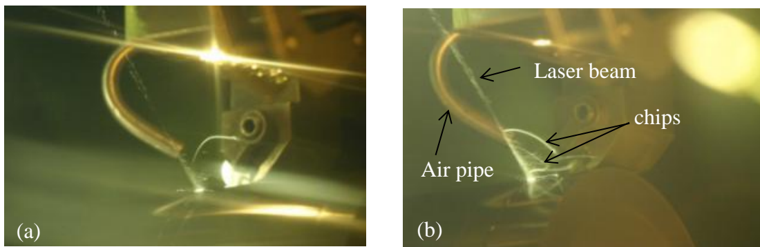
Figure 2.10- a) Laser beam hitting the surface to be machined, b) Laser beam hitting some chips causing them to ignite
