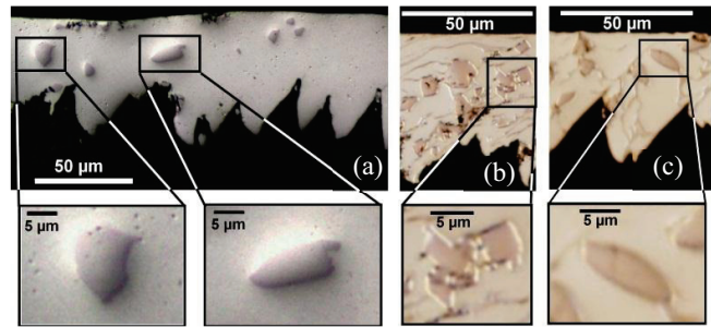
Figure 10 Chip morphologies, (a) particles not broken at T_s=1000^\circ\text{C} , v_c=100 m/min with LAM, (b) broken particles at RT v_c=100 m/min, (c) particle not broken at RT, v_c=170 m/min.
