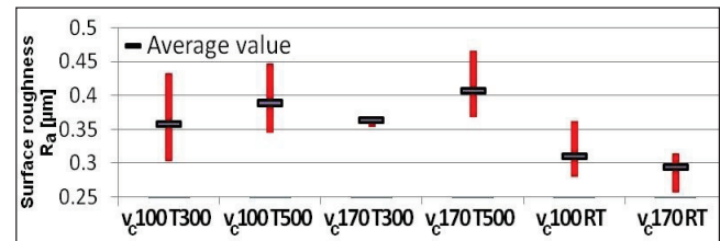
Figure 3 Effect of speed and surface temperature on surface roughness R_a .
