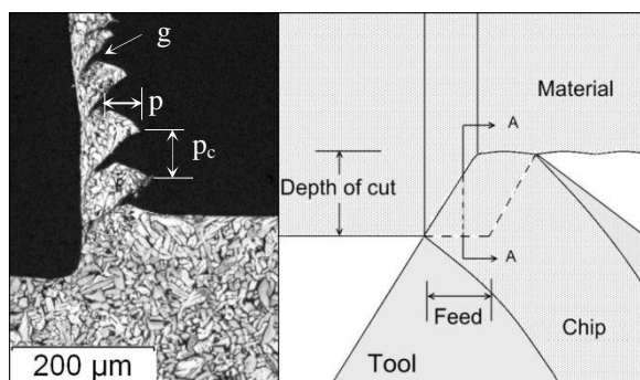
FIGURE 9. SAMPLE AT 500X MAGNIFICATION SHOWING CHIP AT SECTION A-A.
