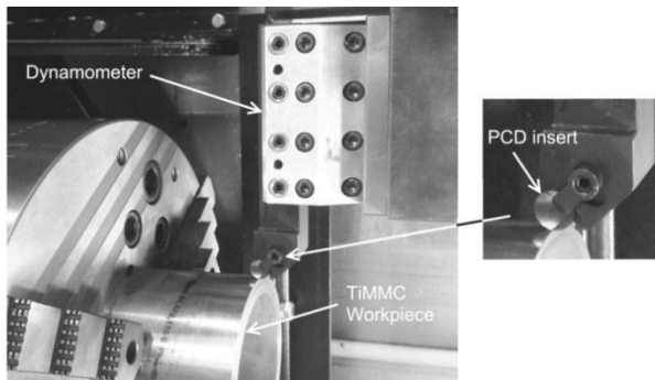
Figure 1: The TiMMC material on the CNC lathe
