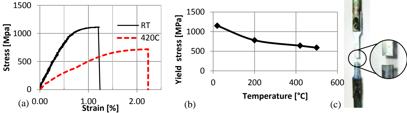
Figure 3, Tensile tests, a) at RT and 420°C, b) RT and HT tests, c) fractured specimen.
