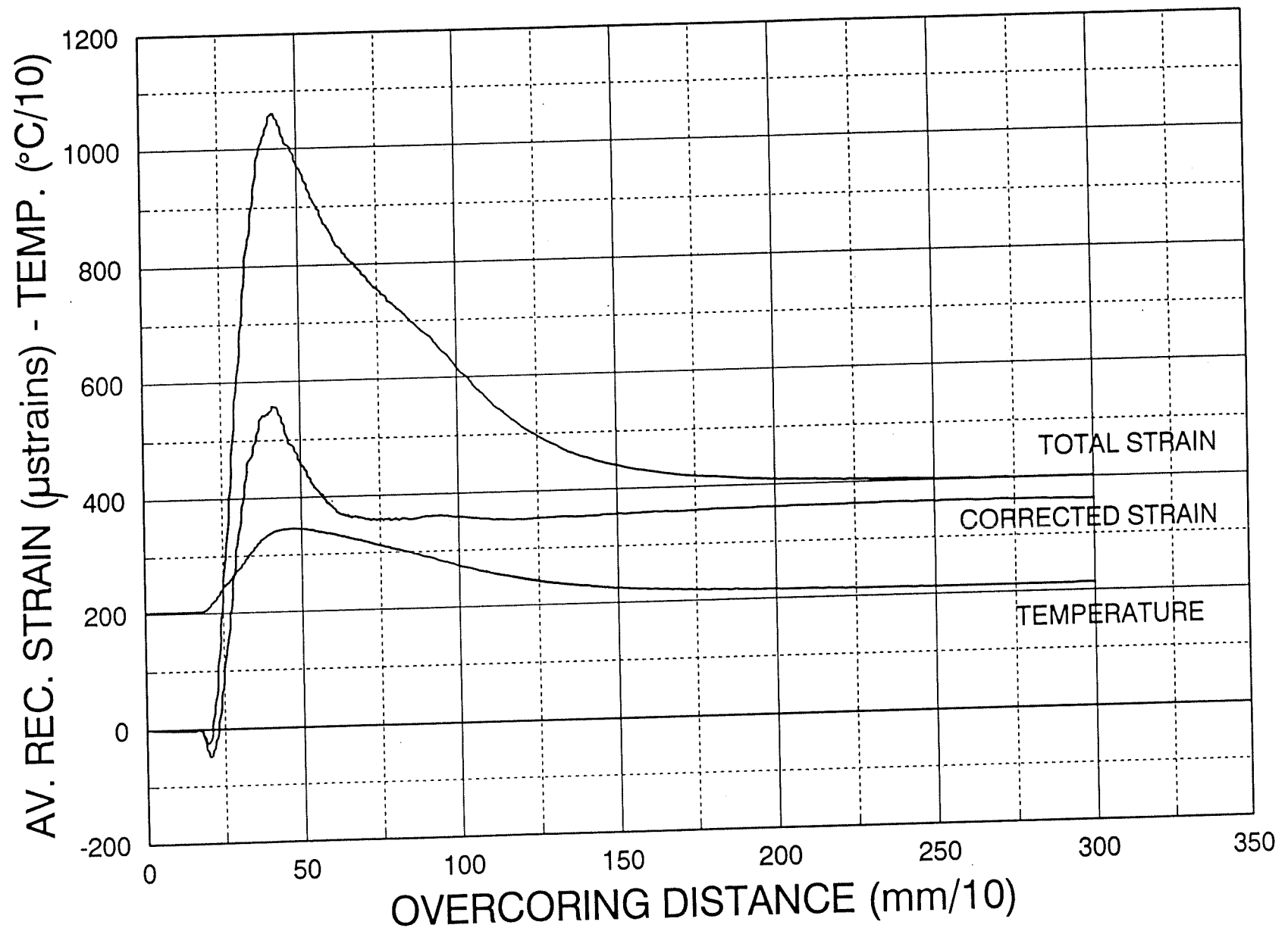
Figure 11: Strain recovery curves from laboratory stress measurement simulations on a rocksalt cylinder (from Corthésy and Gill, 1990)
