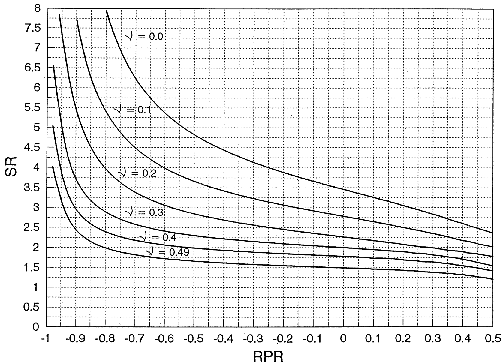
Figure 8: RPR-SR relationships for SR > 2
