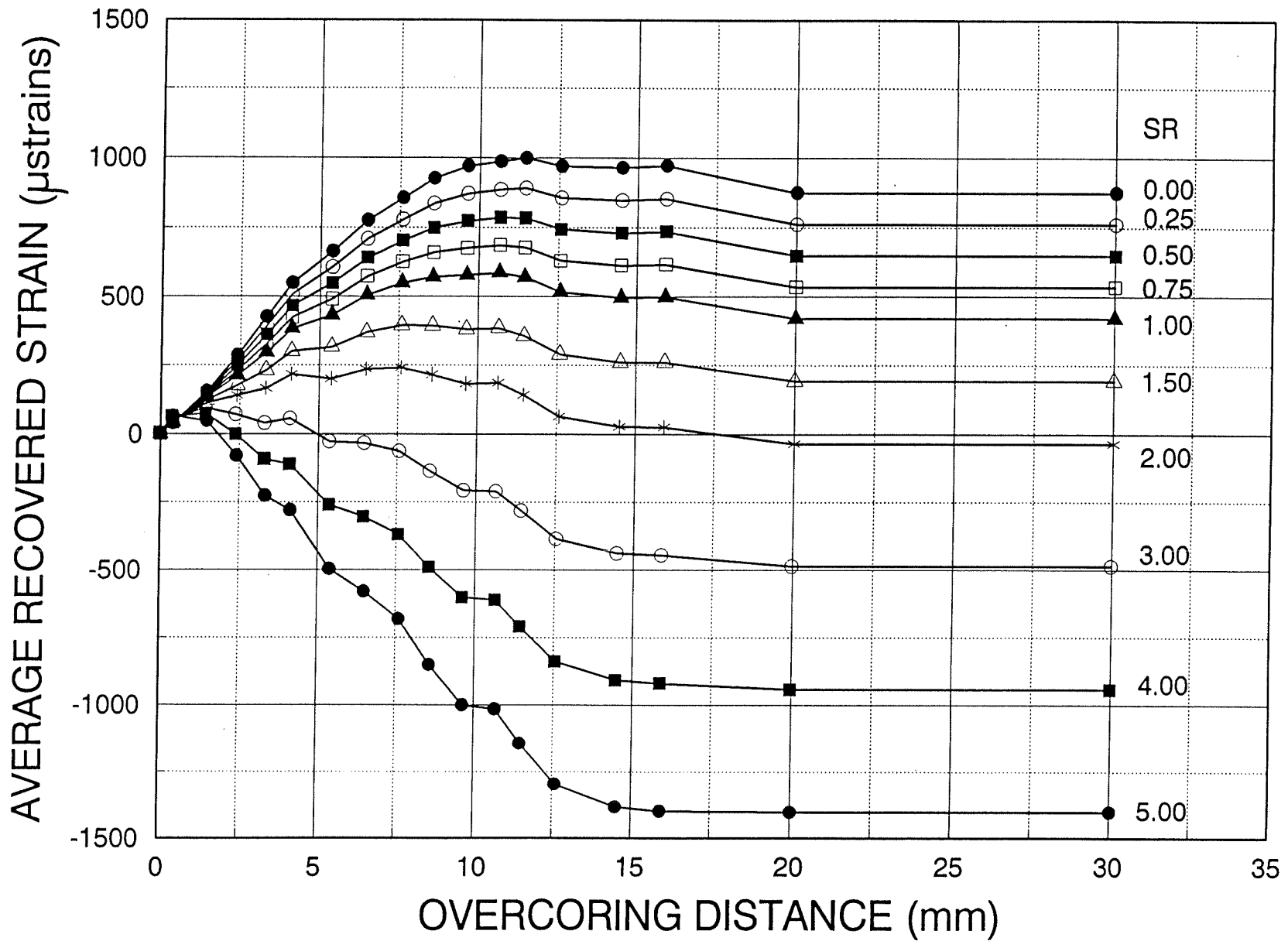
Figure 12: Strain recovery curves from laboratory stress measurement simulations on an epoxy cylinder
