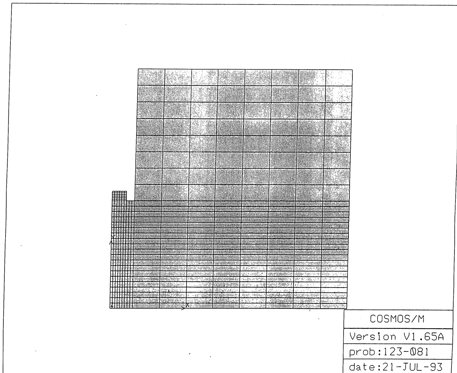
Figure 5: Mesh used for the axisymmetric finite element analyses
