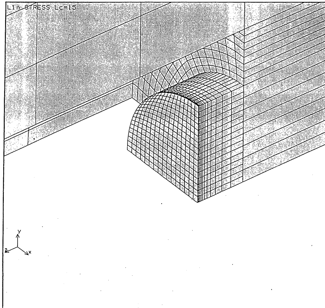
Figure 4: Detail of the 3D mesh used in the finite element analyses
