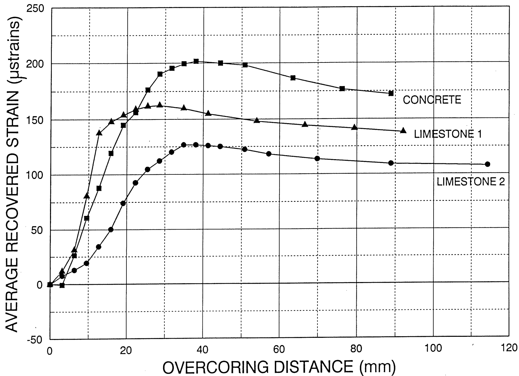
Figure 10: Strain recovery curves from laboratory stress measurement simulations on limestone and concrete blocks (from Fortin, 1981)
