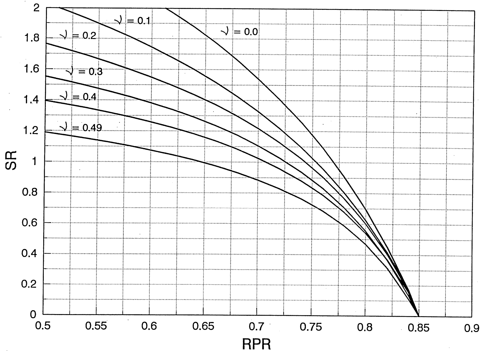
Figure 9: RPR-SR relationships for 0 \leq SR \leq 2
