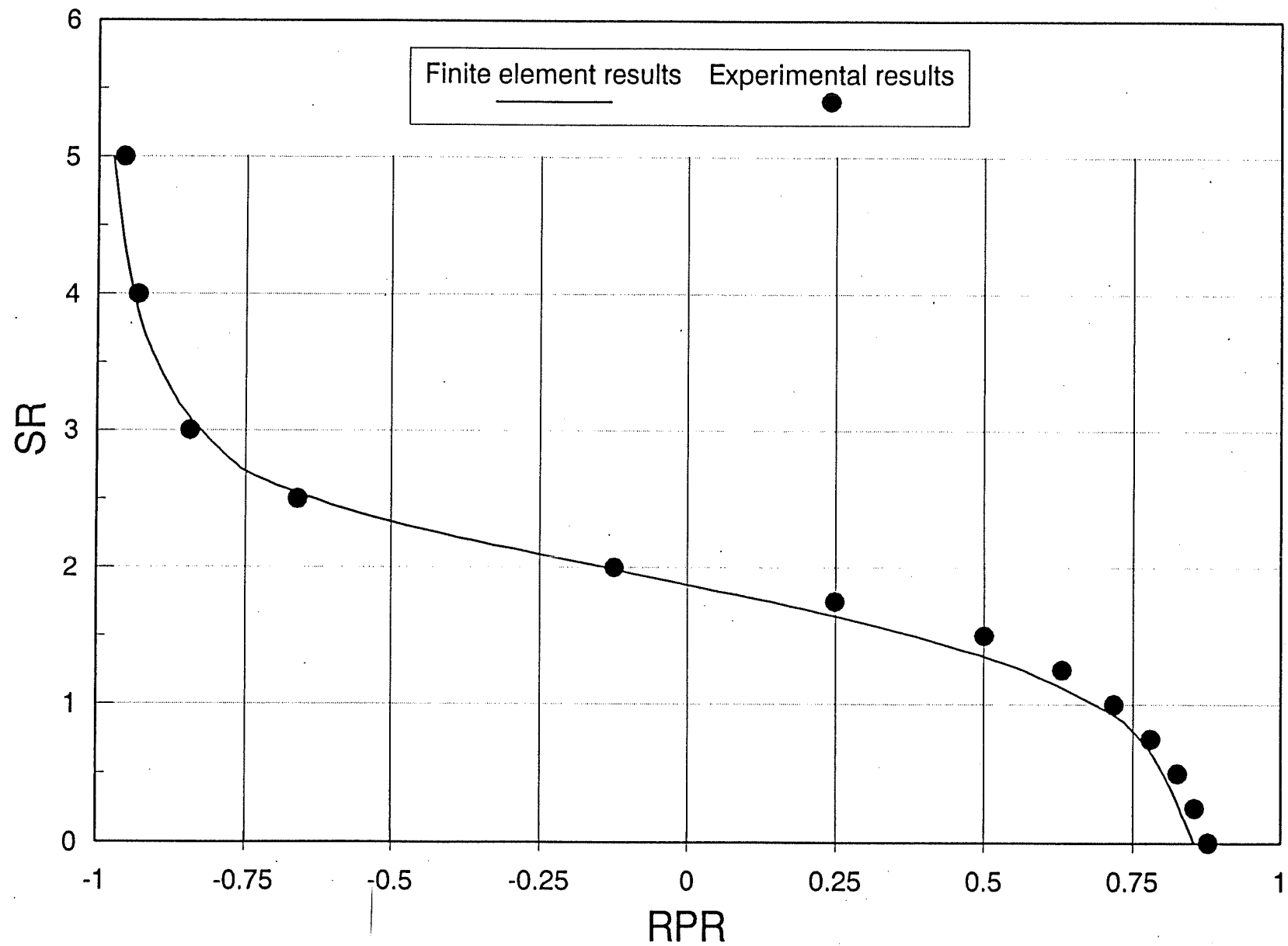
Figure 13: Comparison of the RPR-SR relationships from finite element analyses and stress measurement simulations on an epoxy cylinder
