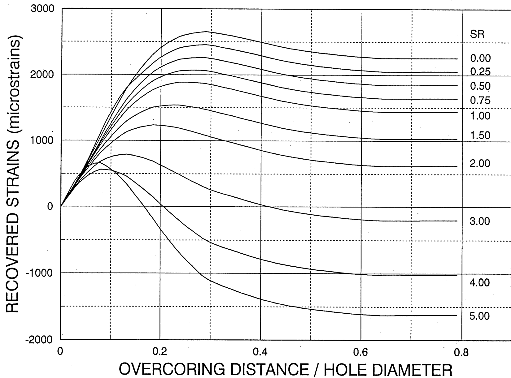
Figure 7: Strain recovery curves for different SR
